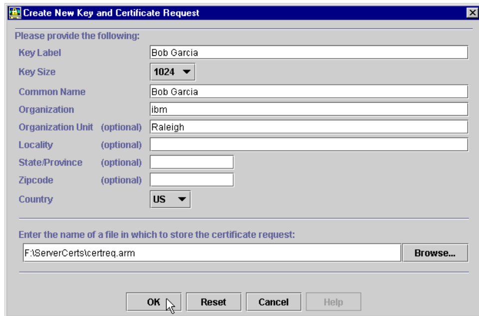
Figure 534. Create New Key and Certificate Request
