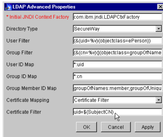
Figure 585. LDAP Advanced Properties window
