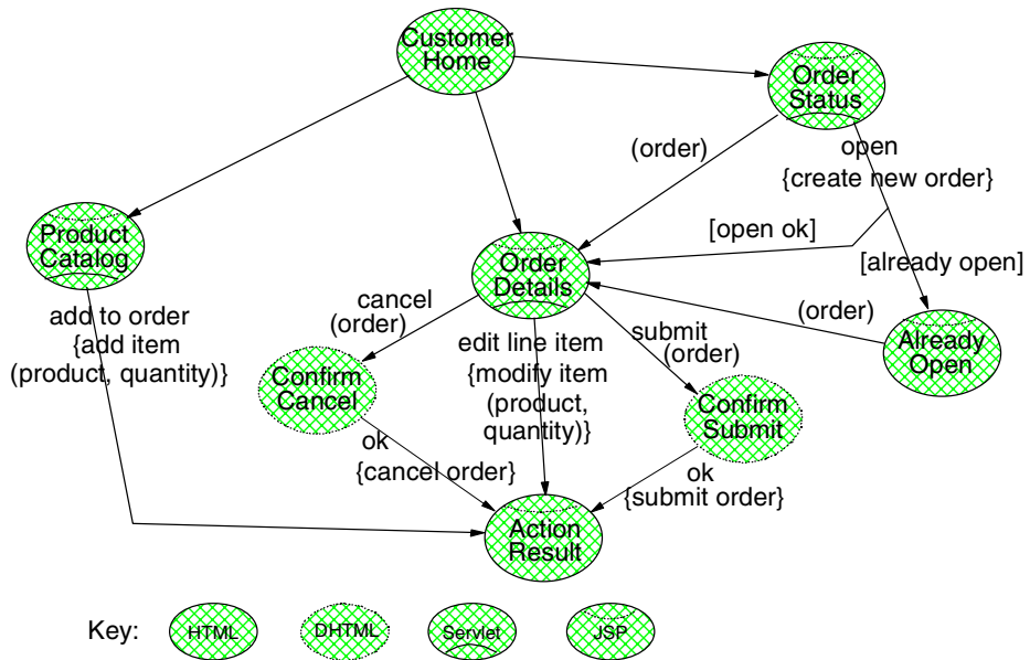
Figure 15. Online buying application STD extended to show display controlled by JSPs
