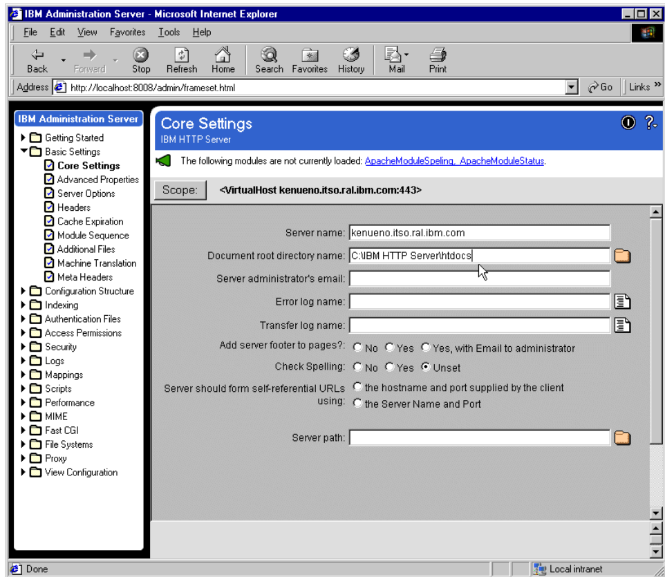
Figure 571. IHS - setting the virtual host document root
