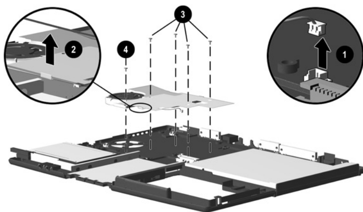
Figure 5-17. Removing the Heat Sink
