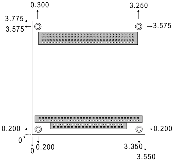
PC/104 & PC/104 Plusmodule dimenstions (inches ± 5%)
