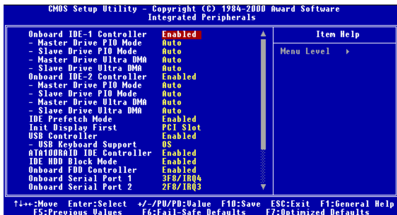
Figure 3-6C. Integrated Peripherals Menu Default Screen (KT7-RAID)
