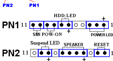
Figure 2-9. The definition of PN1 and PN2 pins
