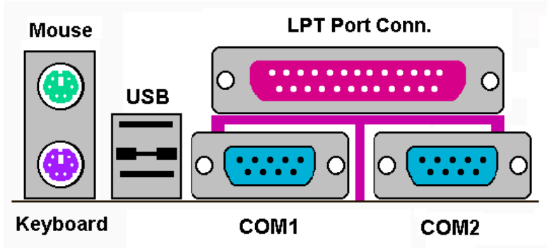
Figure 2-11. KT7/KT7-RAID back panel connectors
