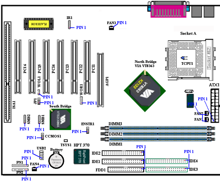
Figure 2-7A. All Connectors and Headers for the KT7-RAID
