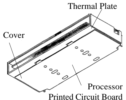
Figure 1: Pentium® II or Deschutes Processor CPU with S.E.C. Cartridge
