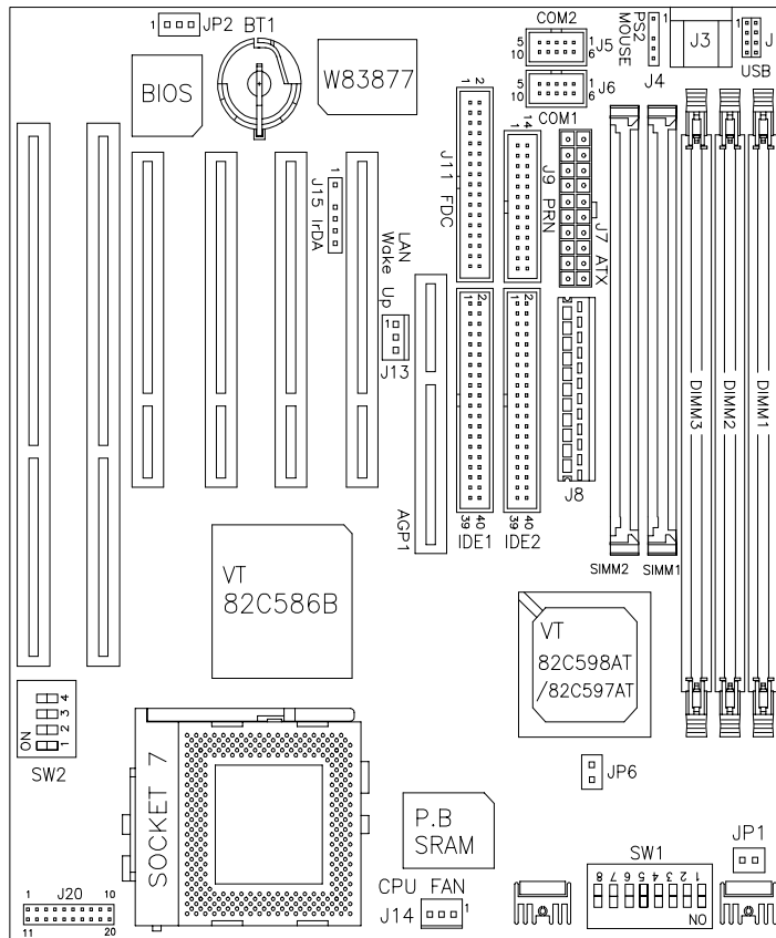
Figure 1: Layout of the AI5VG+ Motherboard
