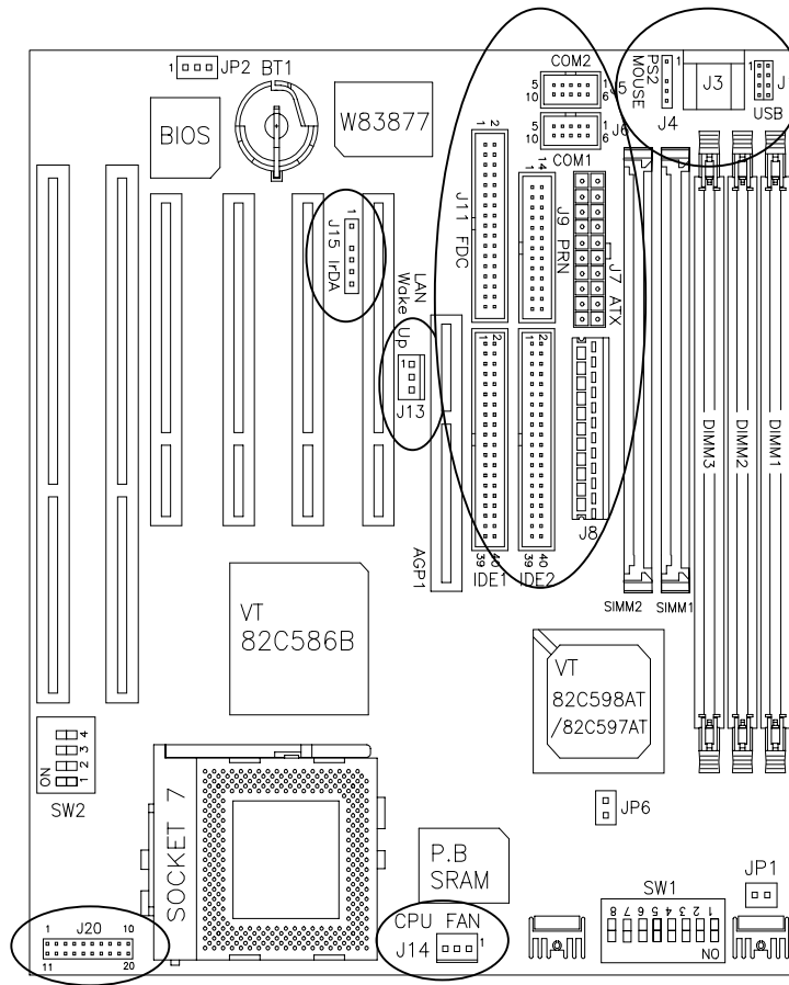
Figure 3: Connector Location on the AI5VG+
