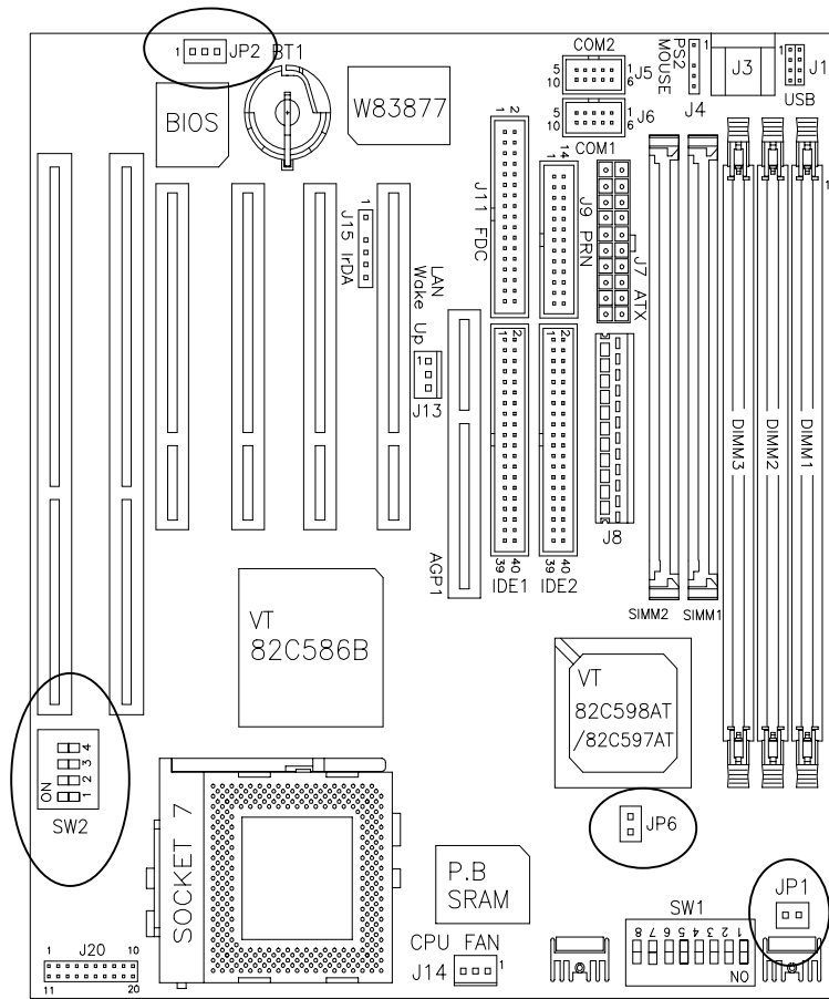
Figure 2: Jumper Locations of the AI5VG+
