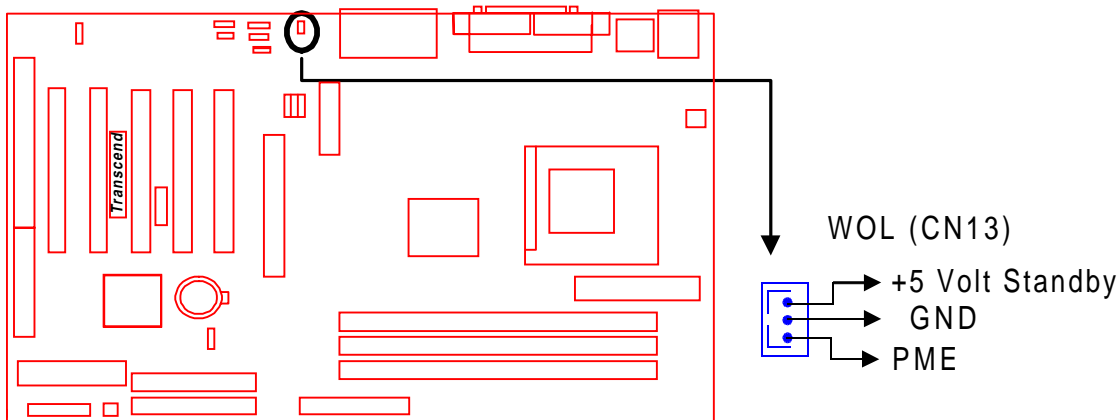
Wake-On-LAN Connector
