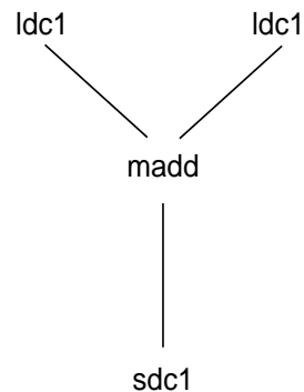
Figure 6-1 A Simple DAXPY Implementation
