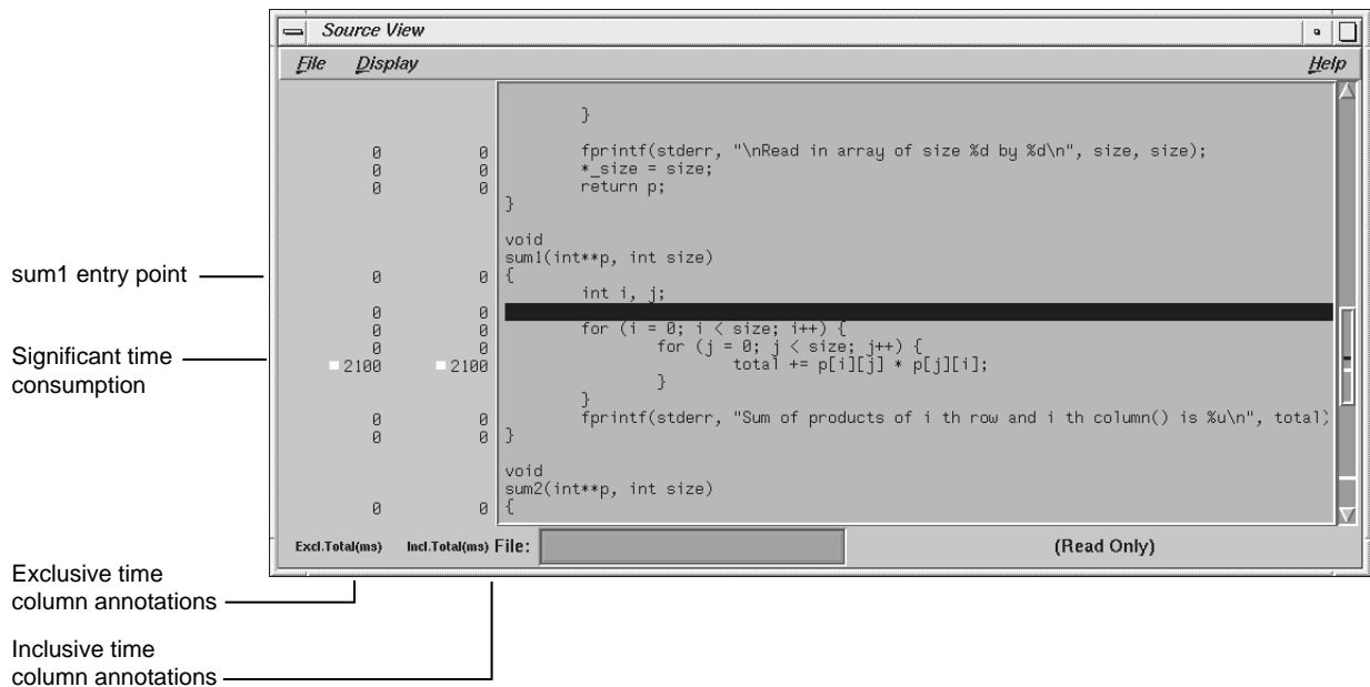
Figure 3-5 Source View with Performance Metrics
