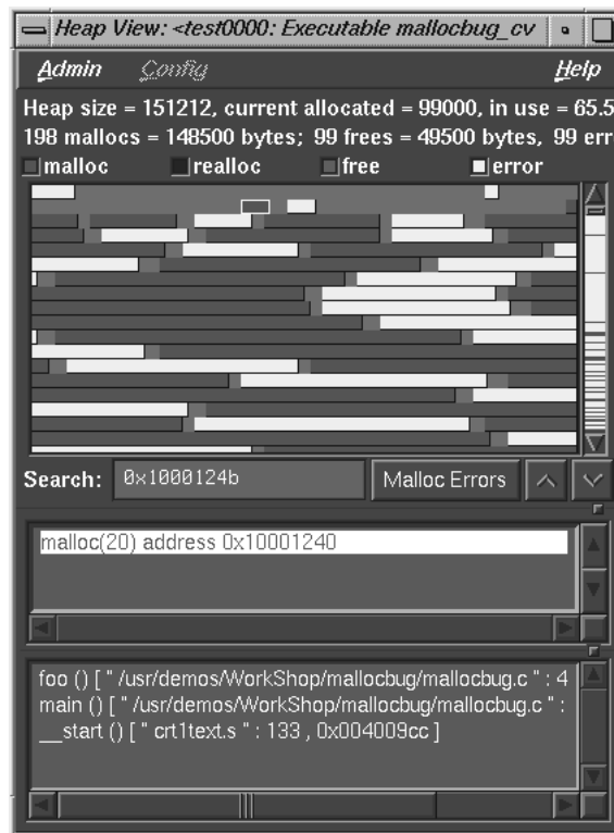
Figure 2-12 Typical Heap View Display Area
