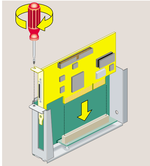
Figure 2-16 Installing the PCI Board
