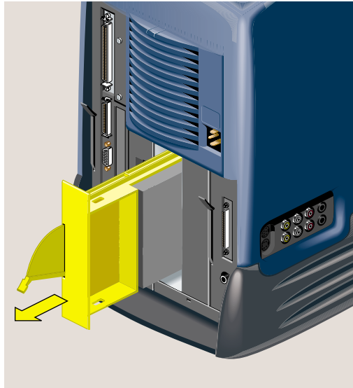
Figure 5-23 Removing the System Drive Module From the Chassis
