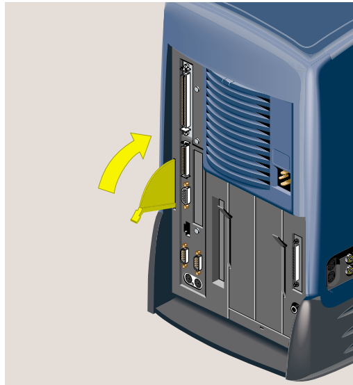
Figure 2-48 Securing the System Module in Place
