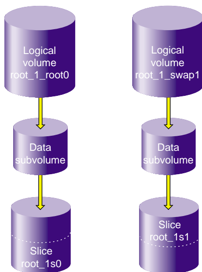
Figure 5-7 XVM System Disk Logical Volumes Before Mirroring
