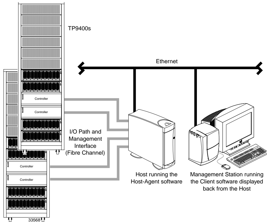
Figure 2-1 Host-Agent Managed Storage Arrays
