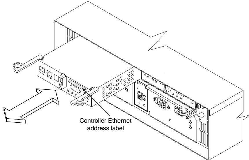
Figure 2-7 Identifying the Controller Ethernet address on the SGI TP9300 RAID Controller
